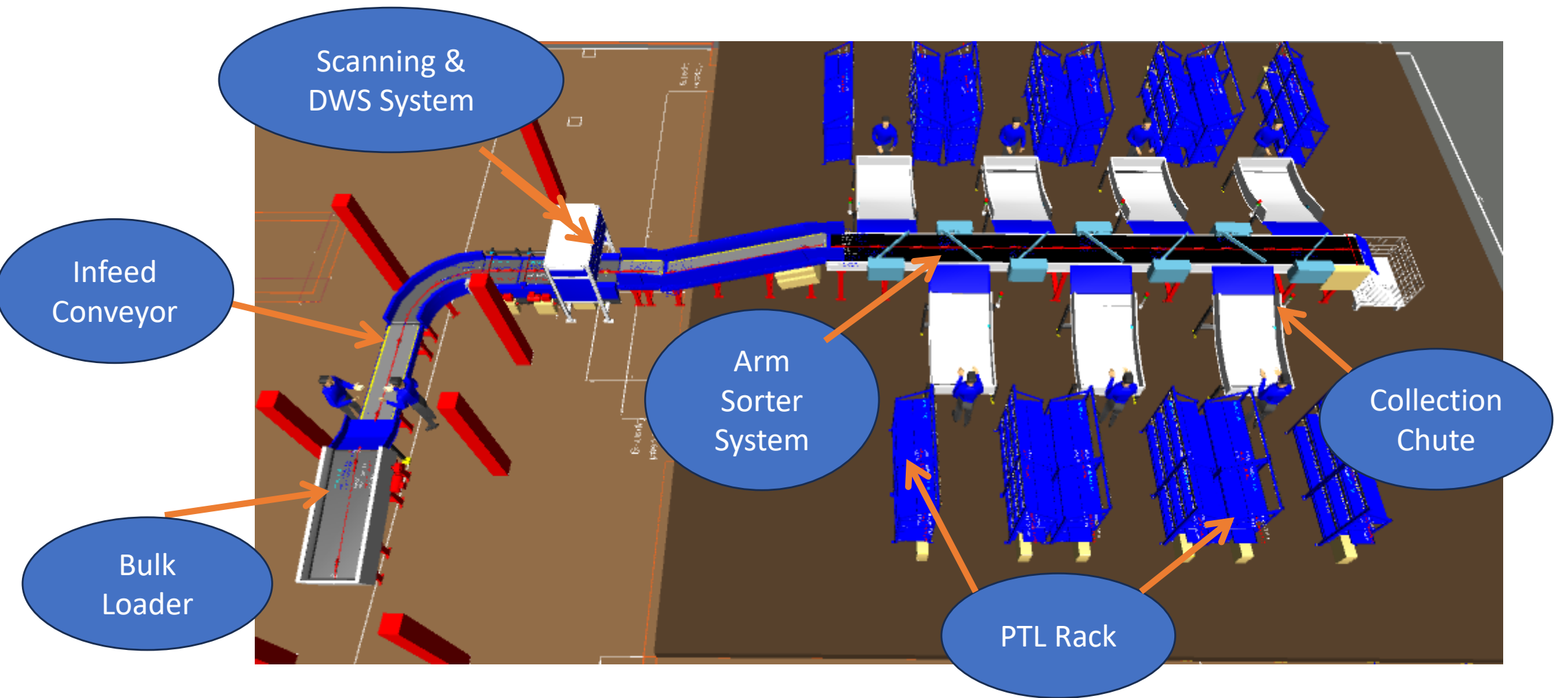
Solution Layout”
